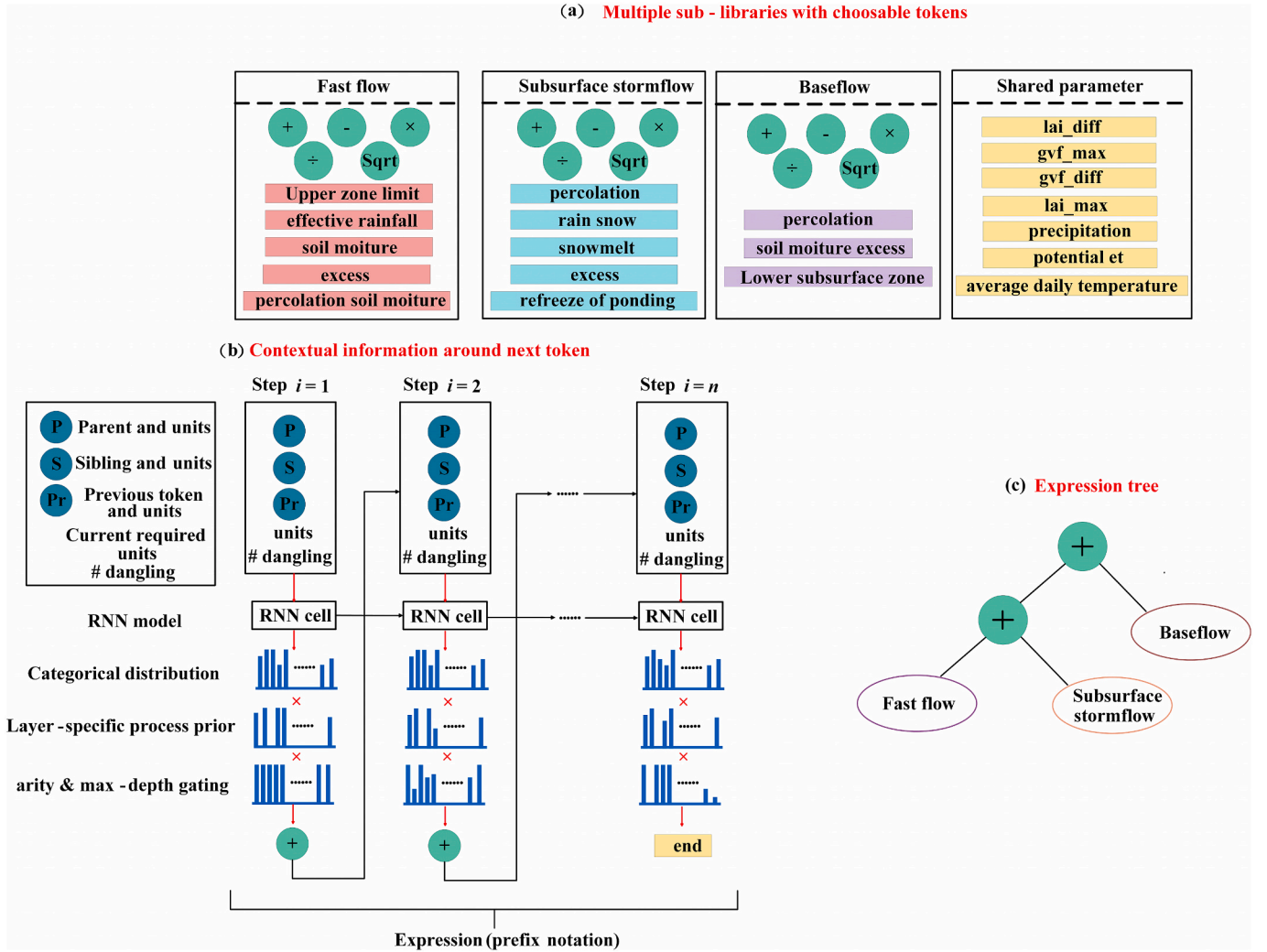
Fig. 3. (a). Includes three process-specific sub-libraries—Fast flow, Subsurface stormflow, and Baseflow—as well as a Shared-parameter sub-library. (b). Illustrates the expression sampling pipeline from the RNN: starting from the contextual inputs and the categorical distribution, then applying the arity & max-depth gating and the layer-specific process prior, until the prefix-form expression is produced. (c). The final expression is organized in a tree structure, with the root node as an additive aggregator and three subtrees corresponding to fast flow, subsurface storm runoff, and base flow, respectively, to achieve a structured and explicit decomposition of the total runoff.
