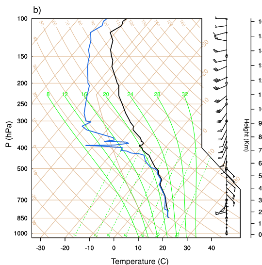
FIG. 8. (a) The 500-hPa level geopotential (height contoured at 30-m intervals) for 1200 UTC 12 Sep 2013 and (b) the sounding from Denver, Colorado, at the same time. Red dot in (a) indicates the geographic location of Denver. Data in (a) are from the National Centers for Environmental Prediction (NCEP) final operational global analysis (FNL).
