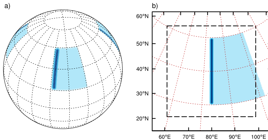
FIG. 1. Horizontal domains for the (a) HiRAM and (b) WRF simulations. In both panels, the blue shaded regions represent the continents, with the mountain ridge in darker blue. The dashed-line box in (b) is the lateral boundary of the inner (12 km) nested domain. (Cross sections of the mountain ridge are shown in Fig. 10.)
