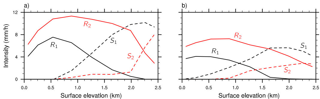
FIG. 14. The 24-h mean intensity of surface rain ( R ) and snow ( S ) of (a) western-slope and (b) eastern-slope extreme events in the control (black) and warmed (red) climate. The subscripts 1 and 2 indicate values for the 1 \times \text{CO}_2 and 2 \times \text{CO}_2 climates, respectively.
