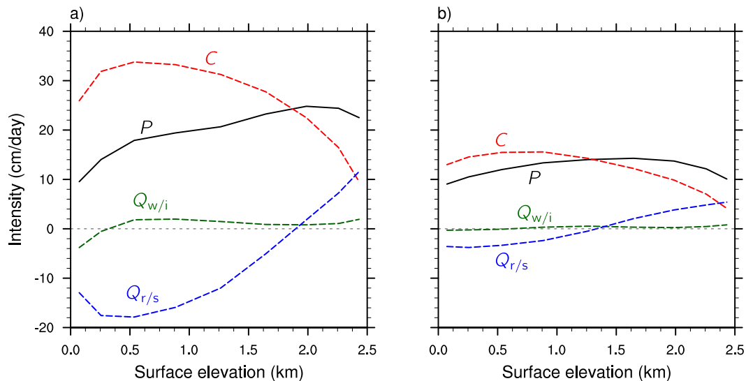
FIG. 12. The 24-h mean intensity of surface precipitation ( P ), column integrated condensation ( C ), and column integrated convergence of rain and snow ( Q_{r/s} ) and of cloud water and ice ( Q_{w/i} ) in the control climate (a) western-slope and (b) eastern-slope extreme events. Negative values indicate divergence.
