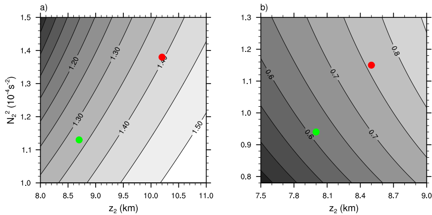
FIG. 11. Vertical velocities w_L in linear mountain waves at height 1.5 km above the middle point of the (a) western and (b) eastern slope as a function of tropopause height z_2 and the static stability of upper troposphere N_2 . Green and red dots indicate the extreme-event mean values in the control and doubled- \text{CO}_2 simulations, respectively. Contour interval is 0.05 \text{ m s}^{-1} .
