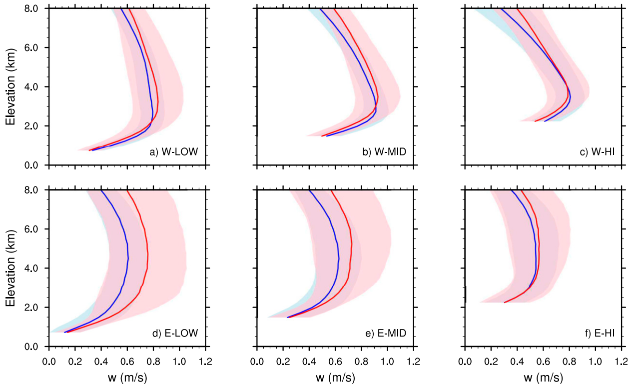
FIG. 9. Profiles of mean \bar{w}_i over the (a)–(c) western and (d)–(f) eastern slopes, for (left) low (0.75 km), (center) middle (1.5 km), and (right) high (2.25 km) surface elevations of the mountains. Blue curves are profiles in the control climate, and red curves are profiles in the 2 \times \text{CO}_2 climate. Event scatter in the control and 2 \times \text{CO}_2 climates is shown by light blue and light pink shading, using one standard deviation of \bar{w}_i in each 10-event set.
