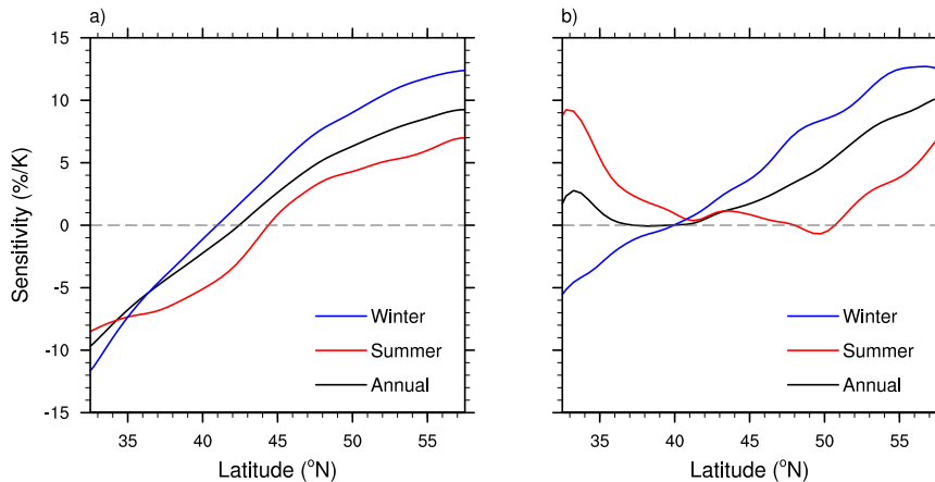
FIG. 2. Sensitivity of annual, summer, and winter mean precipitation over the (a) western and (b) eastern slopes of the mountains.
