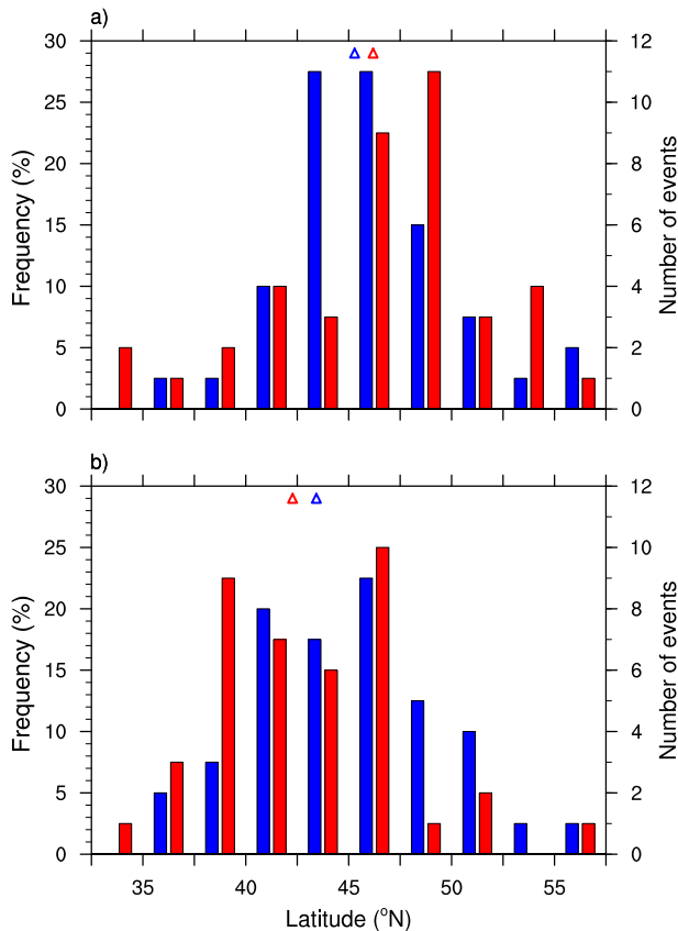
FIG. 4. Histograms of top 40 extreme events in HiRAM simulations on the (a) western and (b) eastern slopes as functions of latitude in the control (blue bars) and 2 \times \text{CO}_2 (red bars) simulations. Blue and red triangles indicate the mean latitudes of extreme events in the control and 2 \times \text{CO}_2 climates, respectively.
