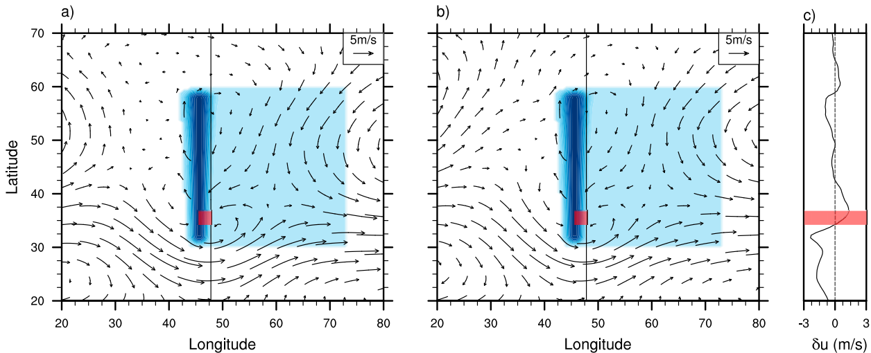
FIG. 3. Mean summertime 850-hPa level wind fields for “significant” precipitation events in the red box (see text) in the (a) control and (b) doubled- \text{CO}_2 climates. (c) The change in zonal wind due to warming at the longitude indicated by vertical black lines in (a),(b). Blue shaded region shows the continent, with the mountain ridge in darker blue.
