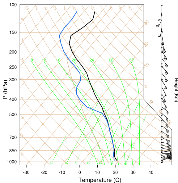
FIG. 7. The sounding and winds in an extreme event plotted on a skew T - \log p chart. The sounding is taken at the same simulation time at the location upstream of the mountain indicated by the blue dot within the red box in Fig. 6b. The black curve is temperature and the blue curve is dewpoint.
