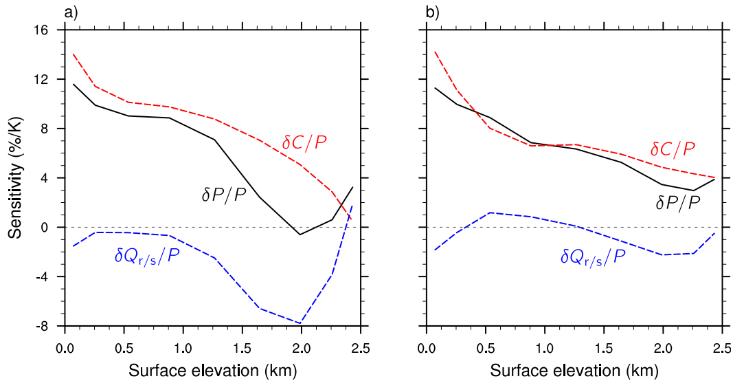
FIG. 13. Contributions of the changes in the column-integrated condensation ( \delta C/P ) and the column-integrated rain–snow convergence ( \delta Q_{r/s}/P ) to the elevational dependence of the sensitivity of precipitation extremes ( \delta P/P ) in (a) western-slope and (b) eastern-slope events.
