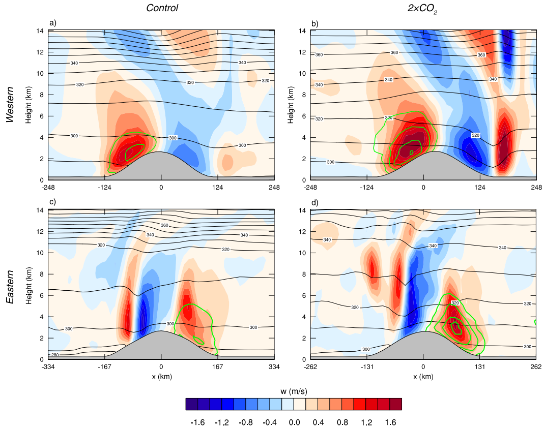
FIG. 10. Snapshots of vertical velocity (color shading) and potential temperature (black contours; K) field on cross sections through the centers of precipitation maxima over the (top) western slopes and (bottom) eastern slopes for (a),(c) extreme events in the control climate and (b),(d) the 2 \times \text{CO}_2 climate. Also shown in green are contours of the condensation rate at contours of 2, 4, 6, and 8 \text{ kg h}^{-1} . These cross sections are taken parallel to the mean wind direction in the lower troposphere. For (a),(b), the winds are nearly from due west; for (c),(d), the winds are from the southwest.
