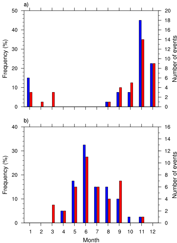
FIG. 5. Histograms of top 40 extreme events in HiRAM simulations on the (a) western and (b) eastern slopes as functions of calendar month in the control (blue bars) and 2 \times \text{CO}_2 (red bars) simulations.
